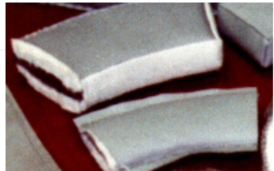
Open ended sectioned examples of side main donut gasket construction with a pinch style design in the forefront and a typical box edge style construction shown in the background. Insulation is layered to provide resilience and durability.
