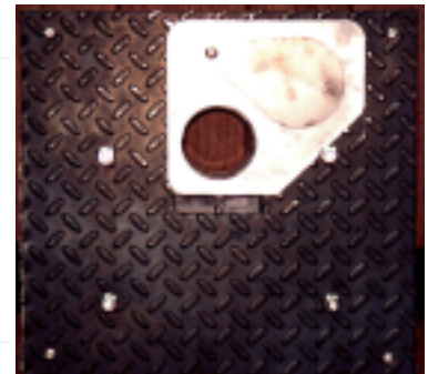
Rectangular exhaust port cover with burner port opening and slide over seal
